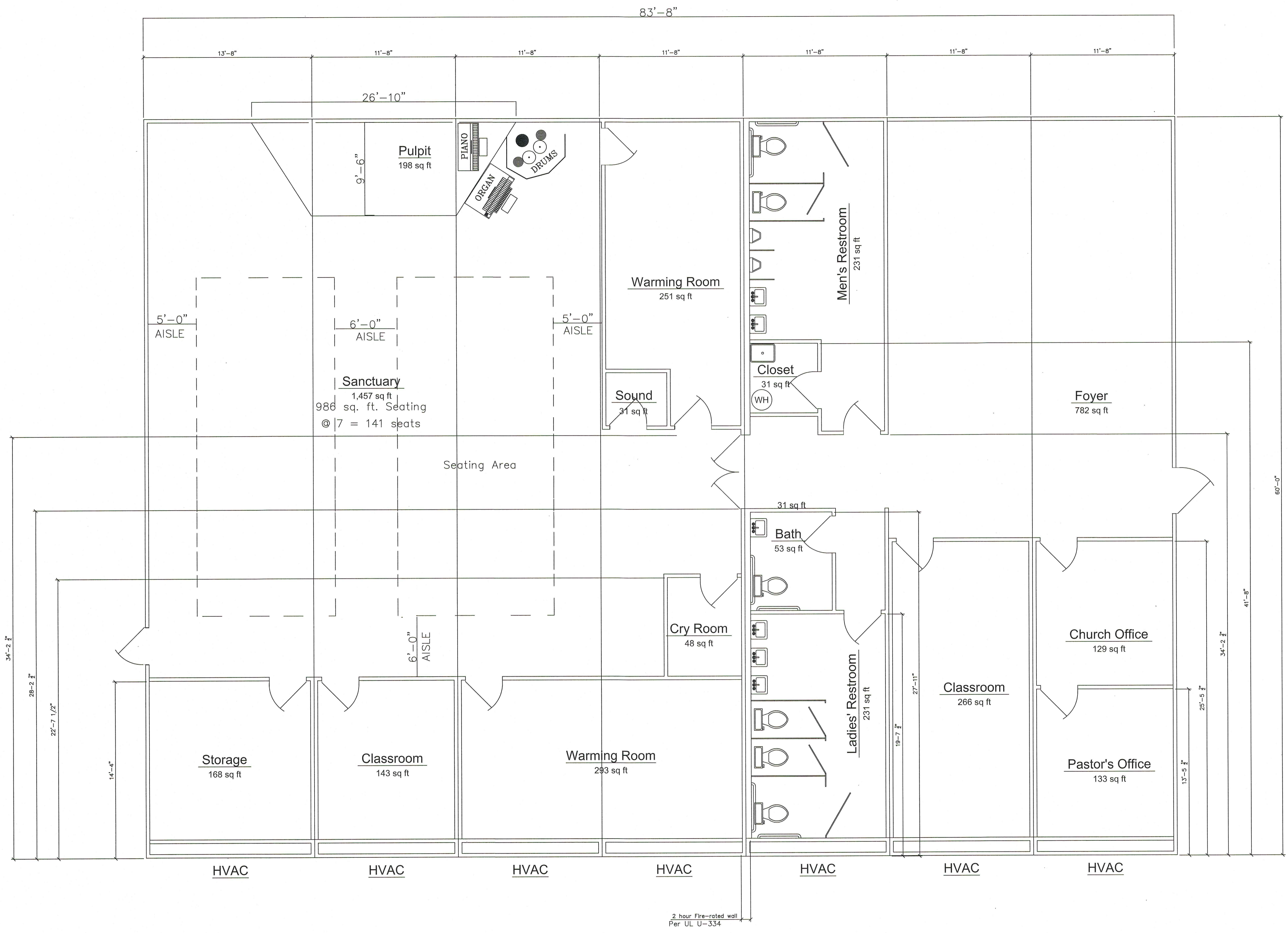
A B-1 FLOOR PLAN SCALE: 1/4" = 1'-0"
