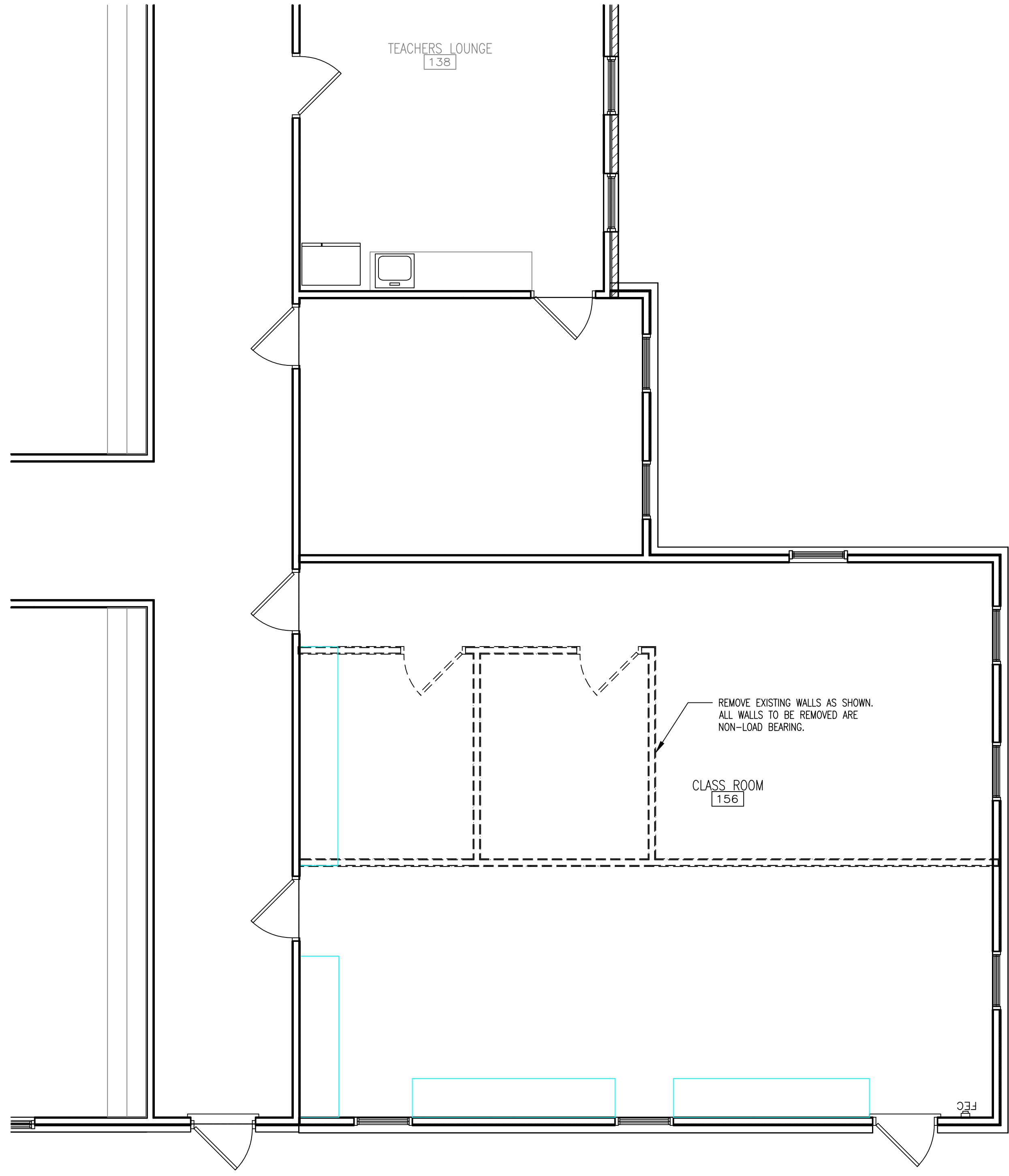
FLOOR PLAN TESTING WING 1/4" = 1'-0"
