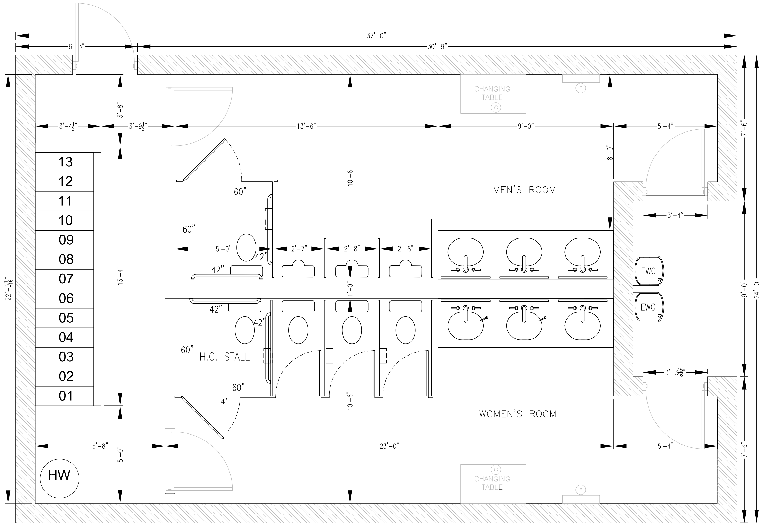
1 FIRST FLOOR PLAN A SCALE: 3/8" = 1'-0"
