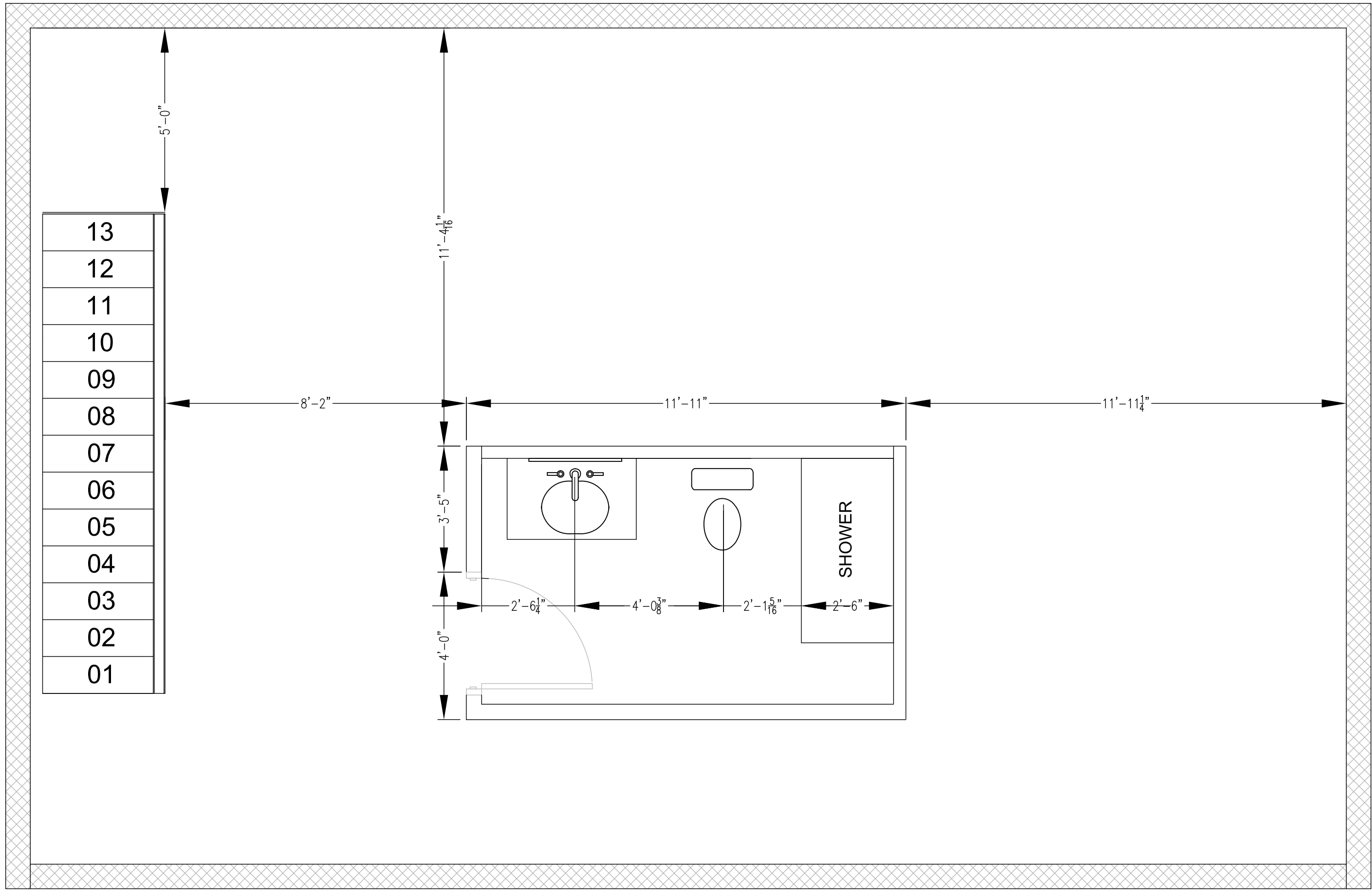
1 A-2 2ND FLOOR PLAN SCALE: 3/8" = 1'-0"
