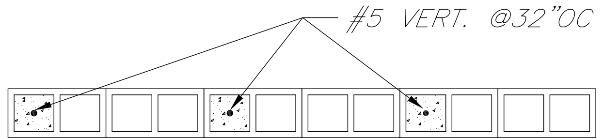
04 CONT. CMU WALL DETAIL S2 SCALE: 3/4" = 1'-0"
