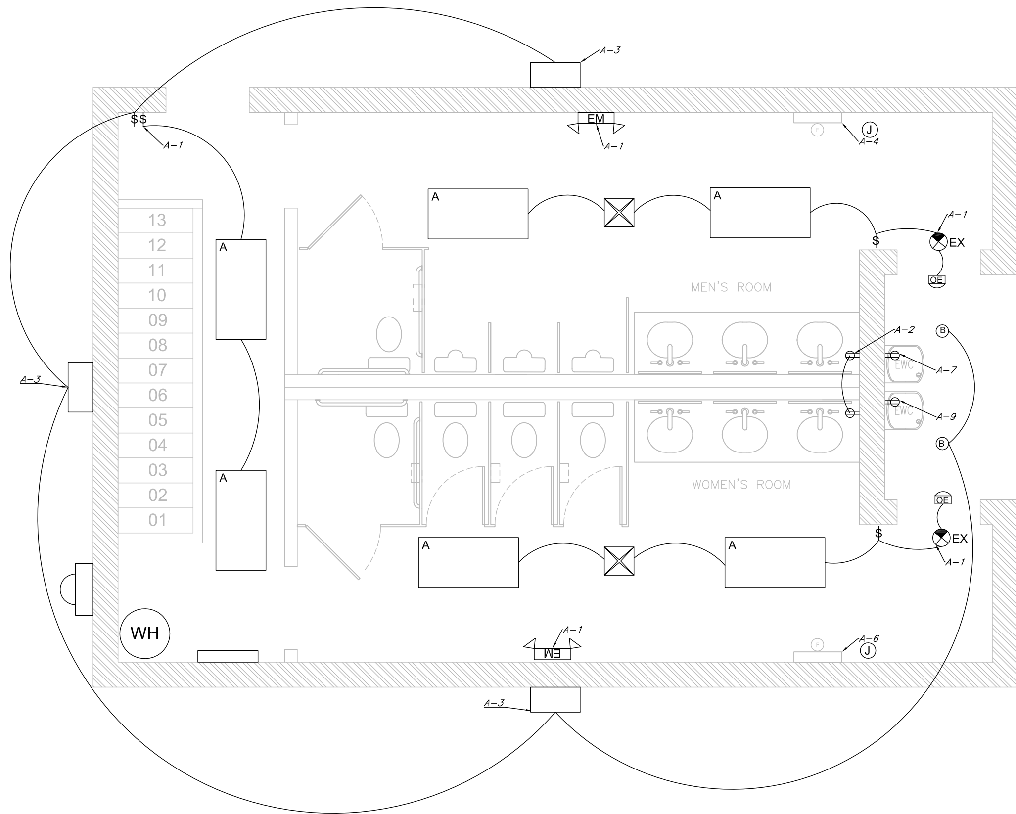
01 LIGHTING PLAN E1 SCALE: 1/4" = 1'-0"
