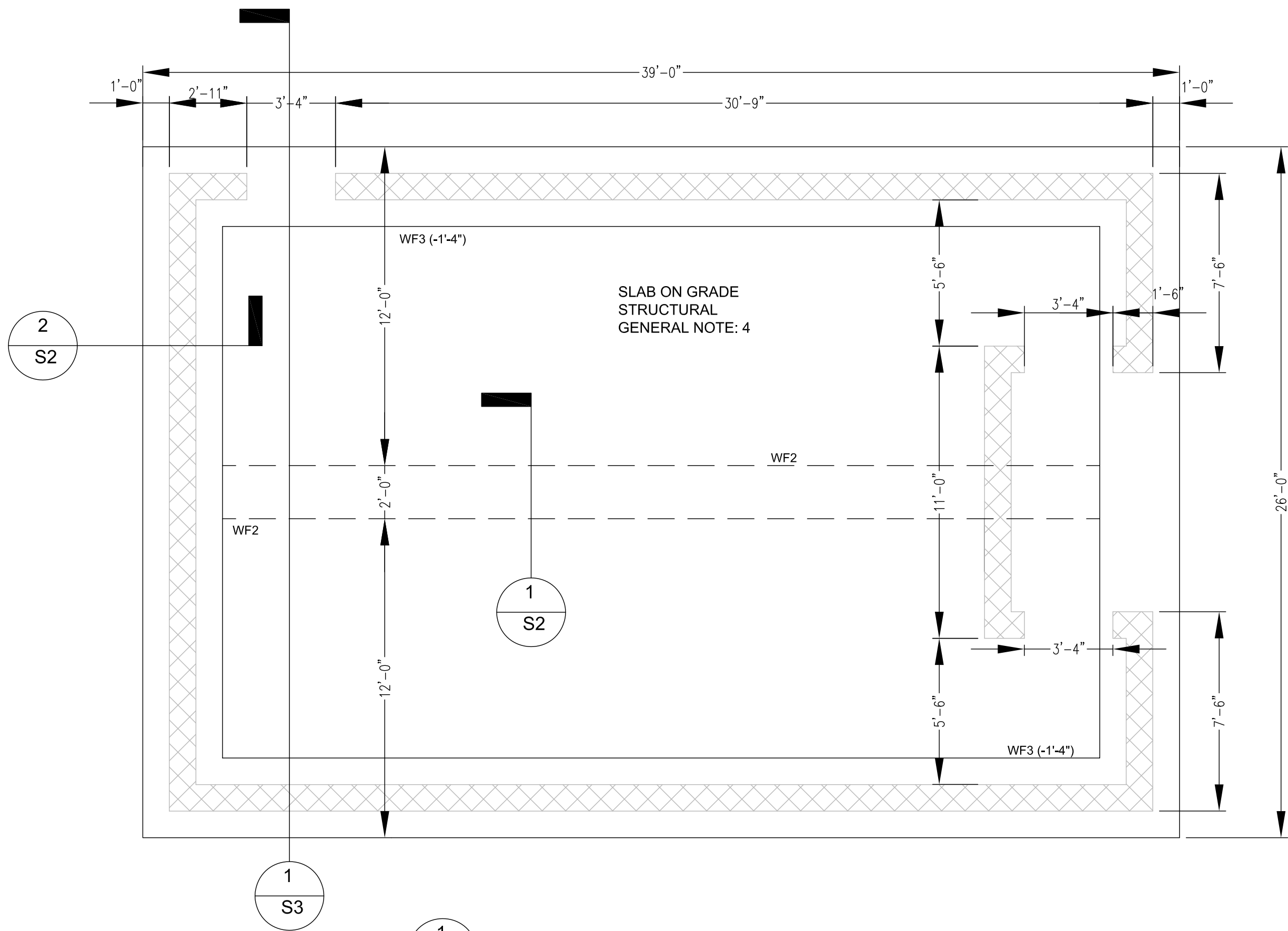
1 S3 FIRST FLOOR PLAN SCALE: 1/4" = 1'-0"
